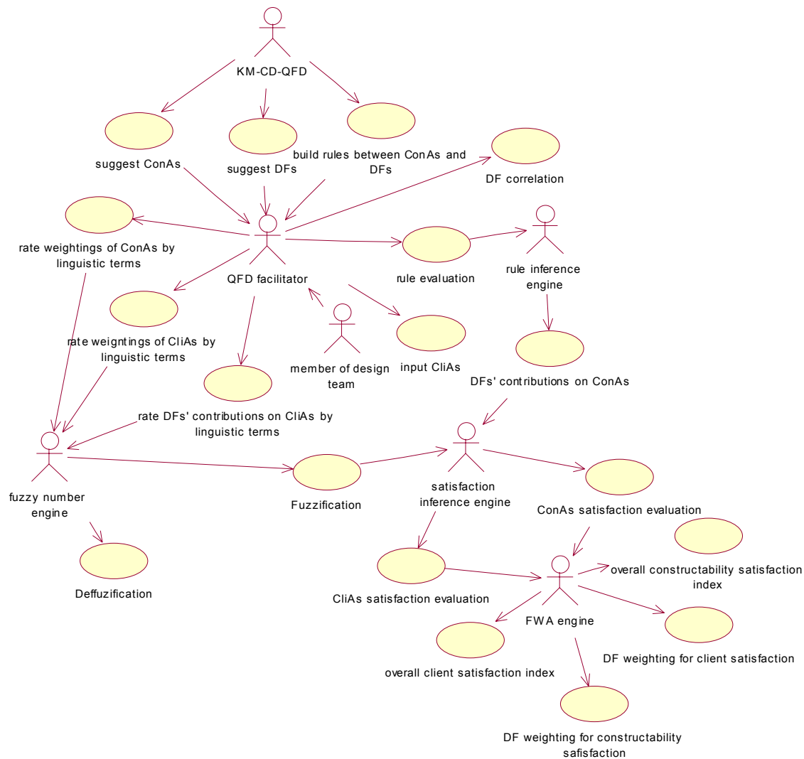
Figure 5 UML-based use case view of intelligent experts
