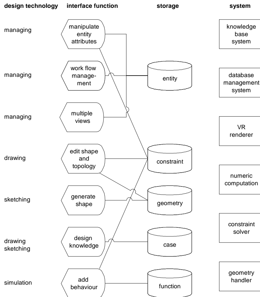
Figure 1: System's architecture
