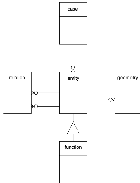
Figure 2: Meta class model
