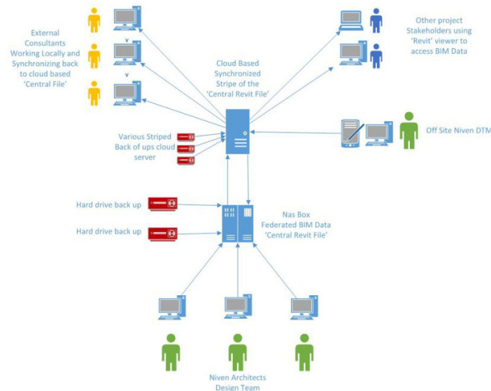
Figure 1. Architecture of the low cost IT network for live BIM in the cloud
