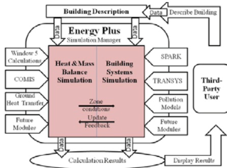
Figure 5 Energy plus flow chart
