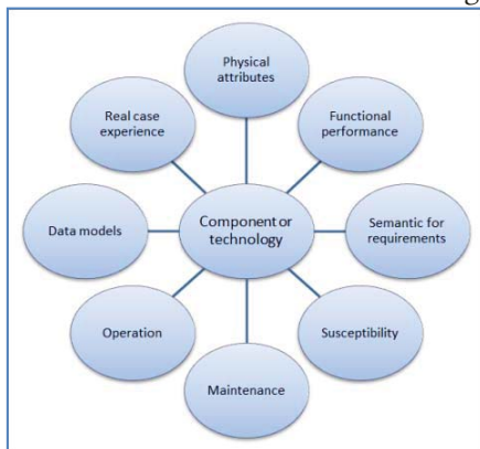
Figure 4 Database schema
