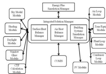
Figure 6 Energy plus modules
