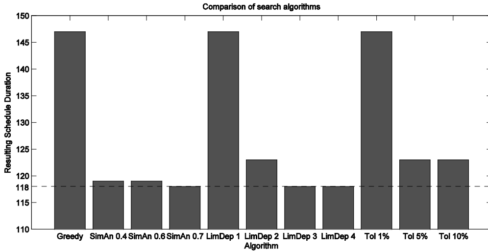
Fig. 10: Result comparison of search algorithms
