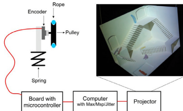
Fig. 3. Scheme of the working installation.
