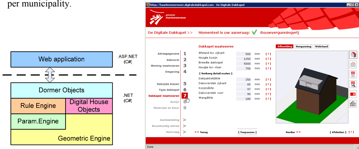
Figure 2: Left: Implementation of The Digital Dormer web application on top of The Digital House API library; Right: sample screenshot of the web application.
