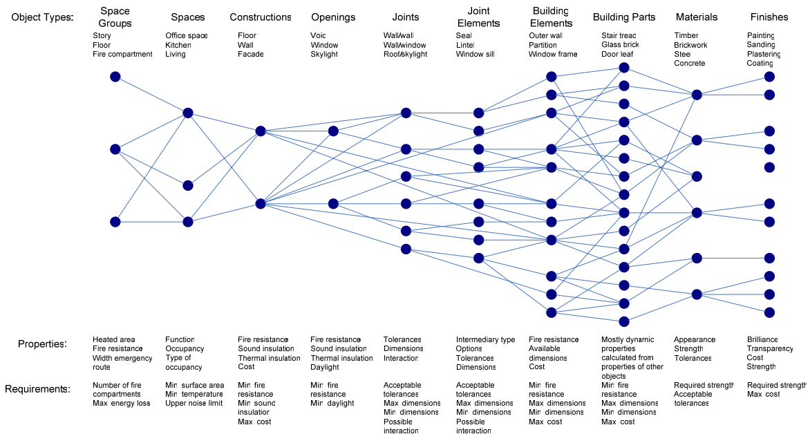
Figure 1: ‘The Digital House’ with examples of object types, properties, and requirements. The picture illustrates the relationships between the 10 groups of object types.
