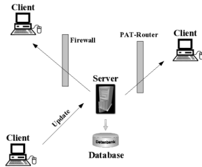
Figure 3. Client-server architecture.
