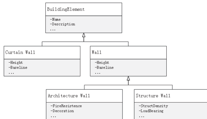
Figure 4: The class inheritance diagram
