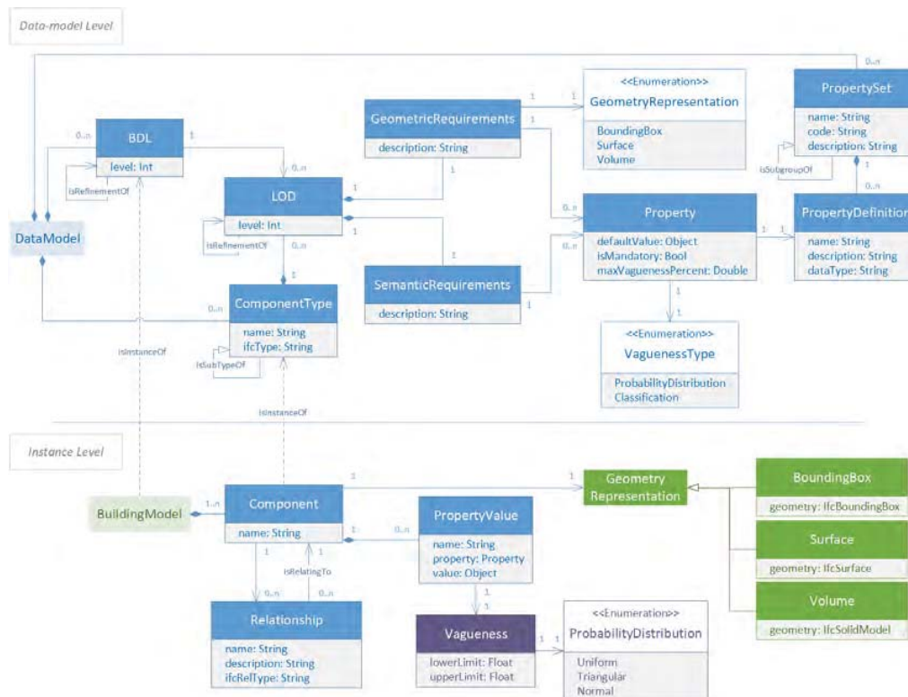
Figure 6: Multi-LOD meta-model (UML diagram)
