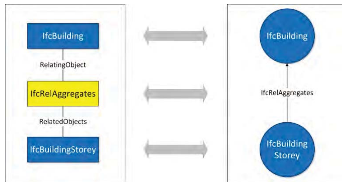
Figure 3: Mapping of classes and relationships
